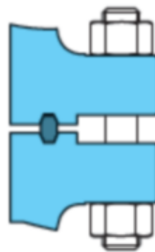
CLASS600–1500 PN 10,0–16,0
